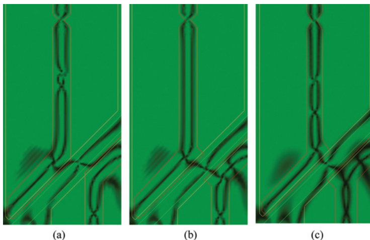
Figure 6. Calculated optical transmittance as a function of the width of the slit: (a) the conventional cell with 8\text{ }\mu\text{m} of the slit width, (b) the proposed cell with 8\text{ }\mu\text{m} of the slit width, (c) the proposed cell with 7\text{ }\mu\text{m} of the slit width. (Figure appears in color online.)
