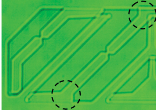
Figure 2. The pattern of the PVA LC cell with defect trap structure. (Figure appears in color online.)
