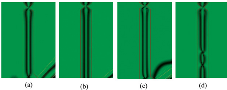
Figure 5. Calculated optical transmittance as a function of the length of the slit: (a) reference ( 20\text{ }\mu\text{m} ), (b) 25\text{ }\mu\text{m} , (c) 30\text{ }\mu\text{m} , (d) 35\text{ }\mu\text{m} . (Figure appears in color online.)
