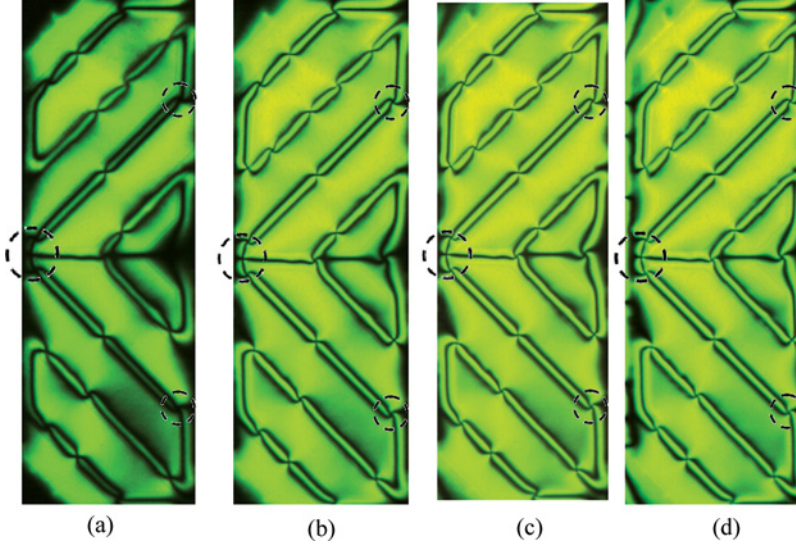
Figure 4. Optical Transmittance of the fabricated PVA LC cell with the defect trap structure: (a) at 4 V, (b) at 6 V, (c) at 8 V, (d) at 10 V. (Figure appears in color online.)
